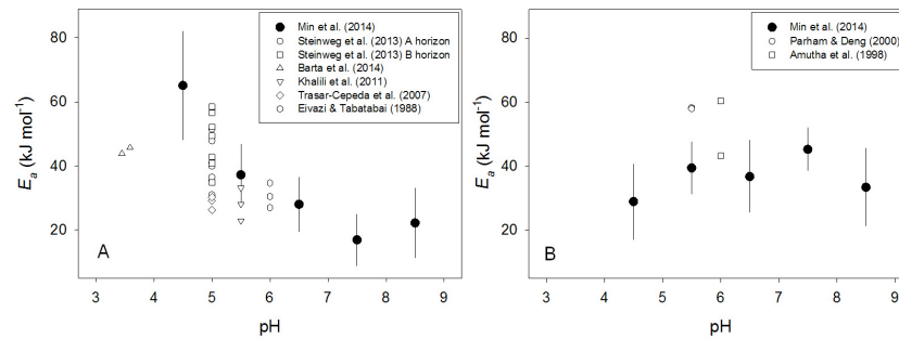
Figure 1. Estimates of intrinsic (closed symbols) and apparent (open symbols) E_a for the BGase/BG reaction (a) and the NAGase/NAG reaction (b). The literature values for apparent E_a are shown at the pH at which the reaction was actually observed, and does not necessarily correspond to the pH of the soils from which the samples were taken. See Sect. 3 for interpretation.
